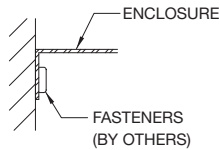
MOUNTING DETAIL OF ENCLOSURE BOTTOM
