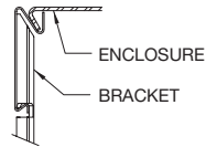
SNAP MOUNTING CHANNEL DETAIL
