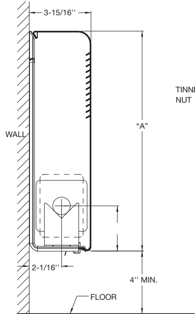
SECTION "X - X" INTERNAL JOGGLE - JOINER
