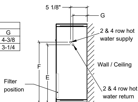
2 & 4 Row Coil Side View
