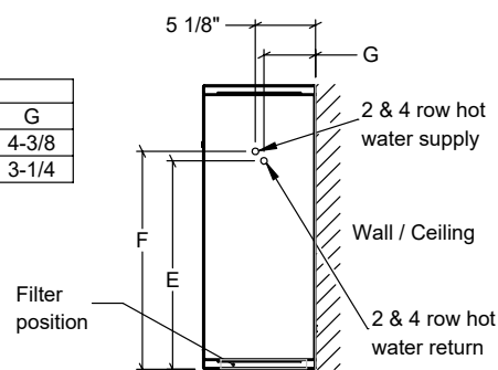
2 & 4 Row Coil Side View
