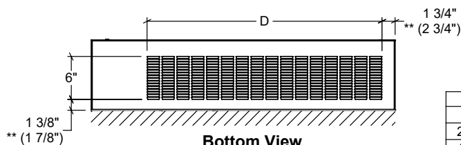
Bottom View
