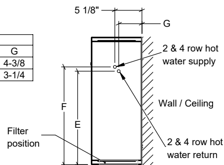
2 & 4 Row Coil Side View
