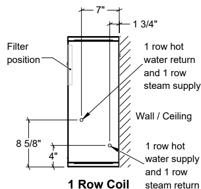
1 Row Coil Side View
