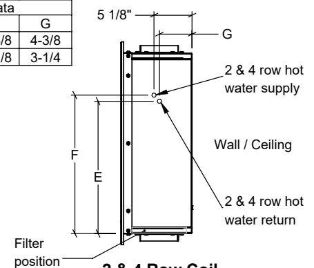
2 & 4 Row Coil Side View
