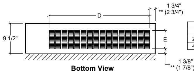
Bottom View
