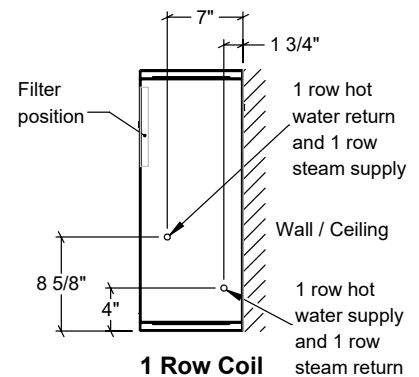
1 Row Coil Side View
