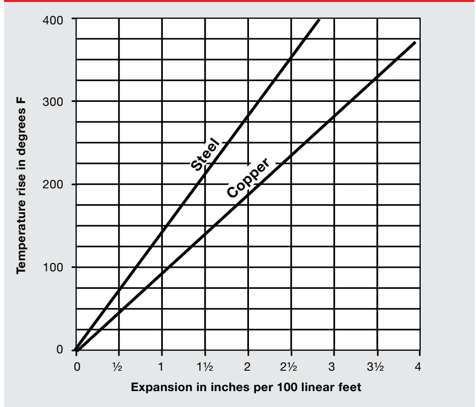
Figure 3 Expansion in steel and copper piping
