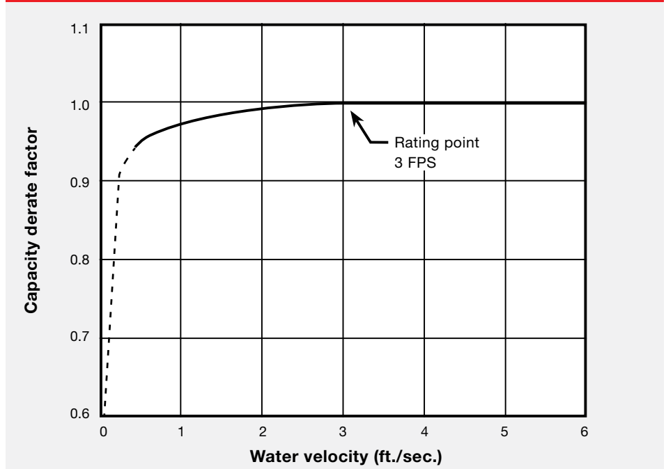
Figure 1 Effect of Water Velocity on Finned Tube Output
