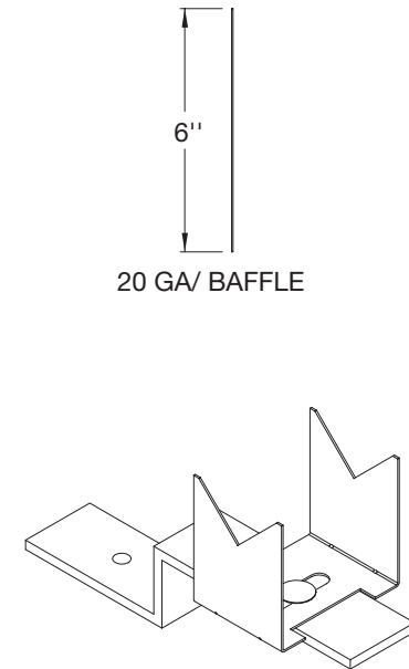
3/16 SUPPORT BRACKET
