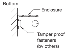
"AP" Access panel with access door, overlapping style only (w/allen key lock)
