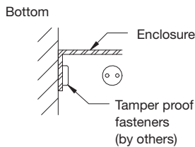
"AS" Removable enclosure section, interlocking style only, no joggles or joiners
