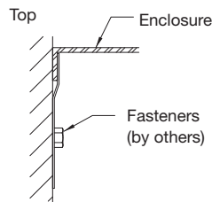
Offset mounting channel detail
