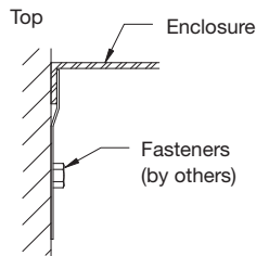
Offset mounting channel detail
