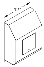
"AC" End cap with access door (w/allen key lock)
