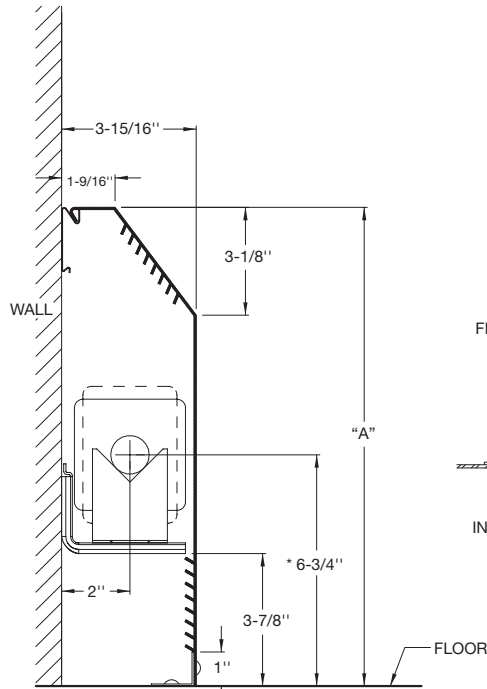
SNAP MOUNTING CHANNEL DETAIL
