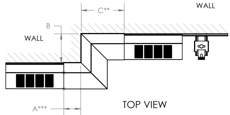
FS5 Z-CORNER RIGHT HAND SHOWN*
