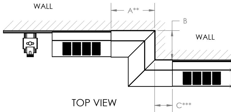
FS5 Z-CORNER LEFT HAND SHOWN*
