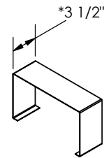
"WT" WALL TRIM STRIP *3-1/2", 5", 7-1/2"
