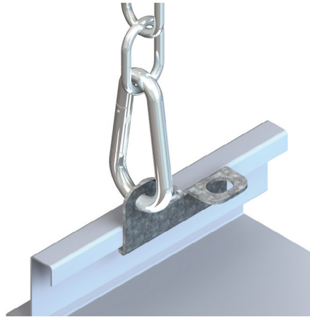
Fixing clips panel connection
